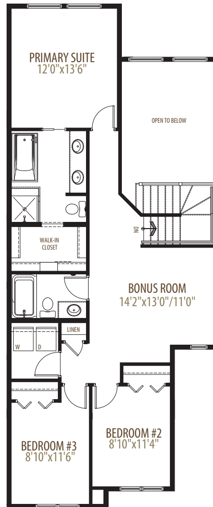
Upper Floor 1,038 sq ft
