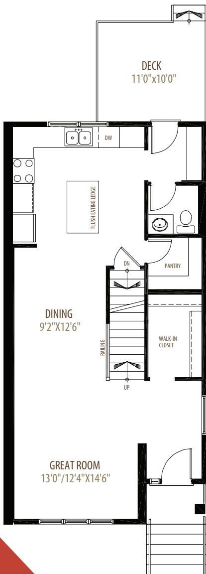
Main Floor 776 sq ft
