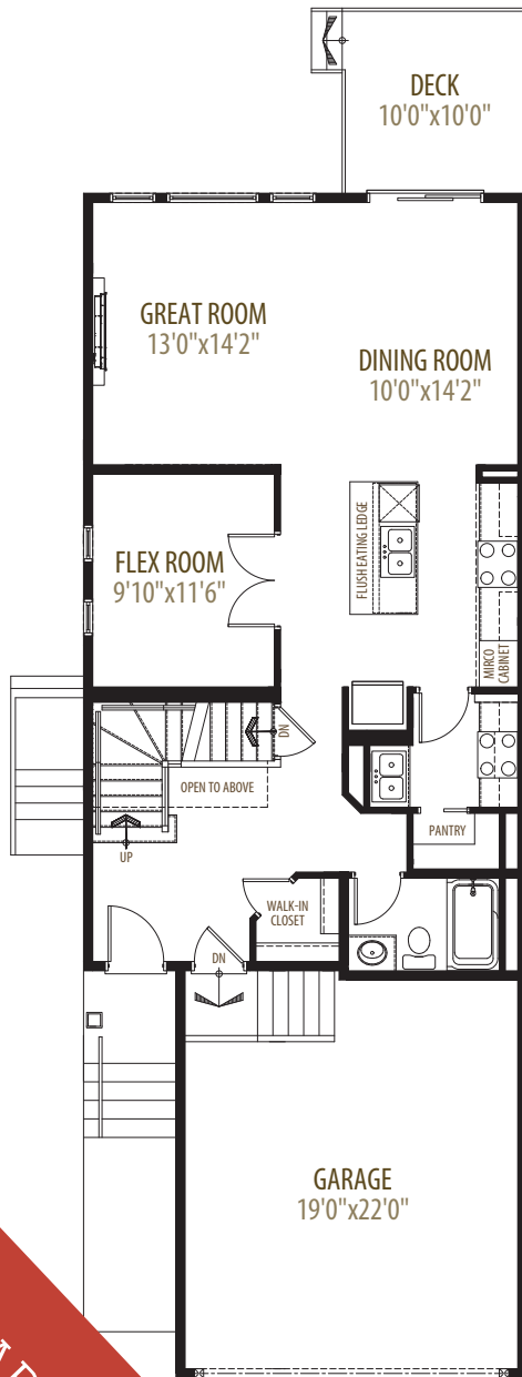
Main Floor 1,014 sq ft
