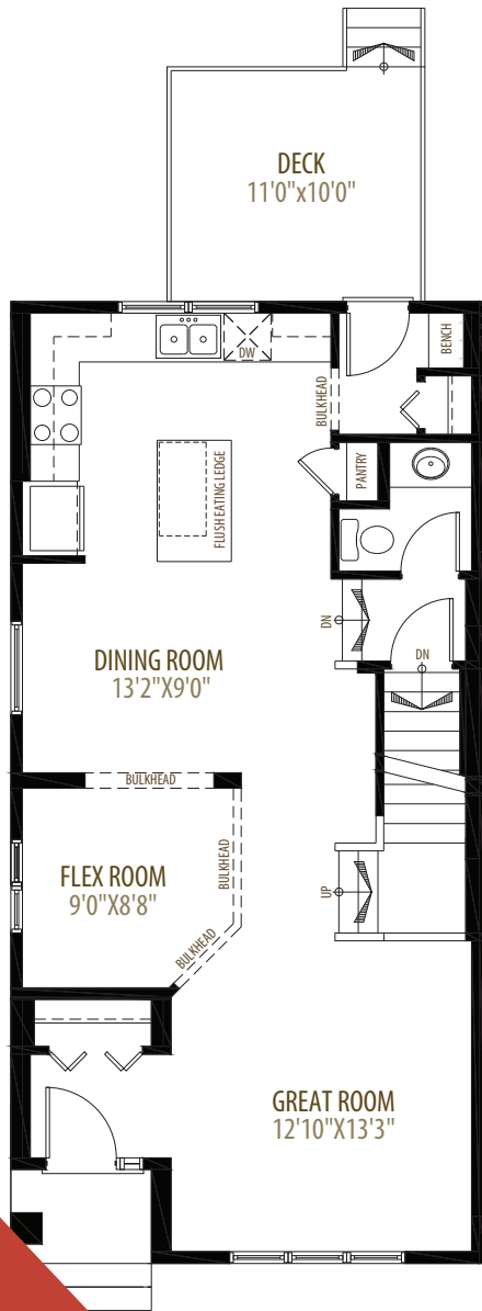
Main Floor 796 sq ft
