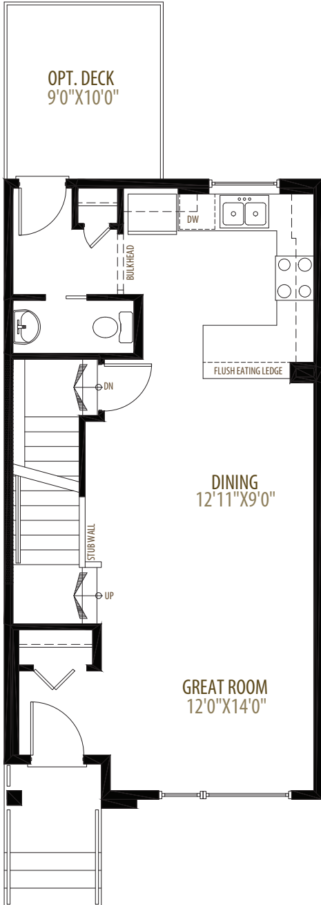
Main Floor 619 sq ft
