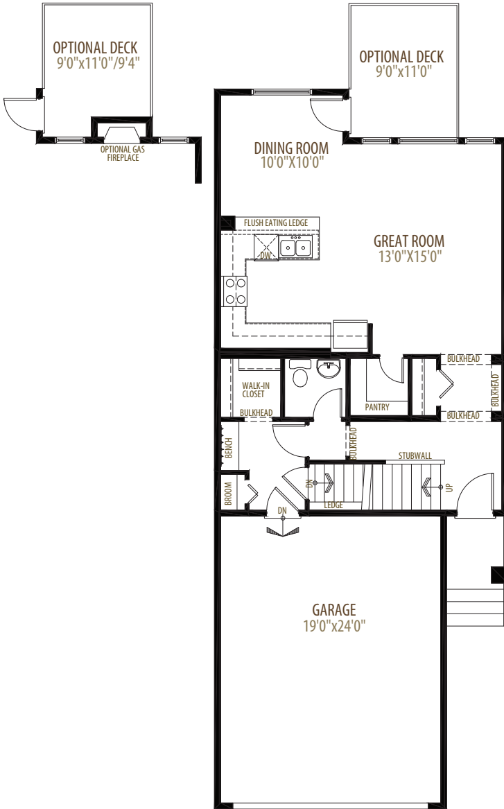
Main Floor 788 sq ft
