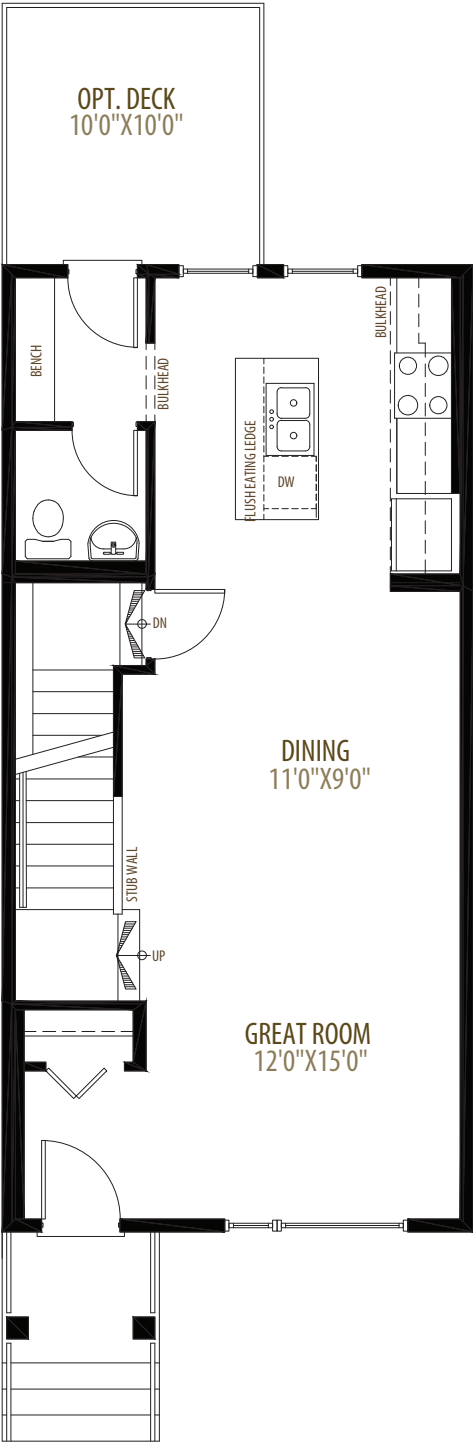
Main Floor 665 sq ft
