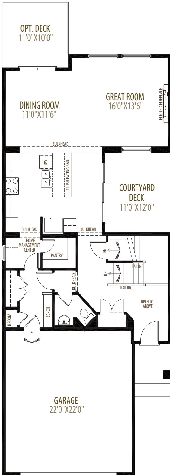
Main Floor 1,035 sq ft
