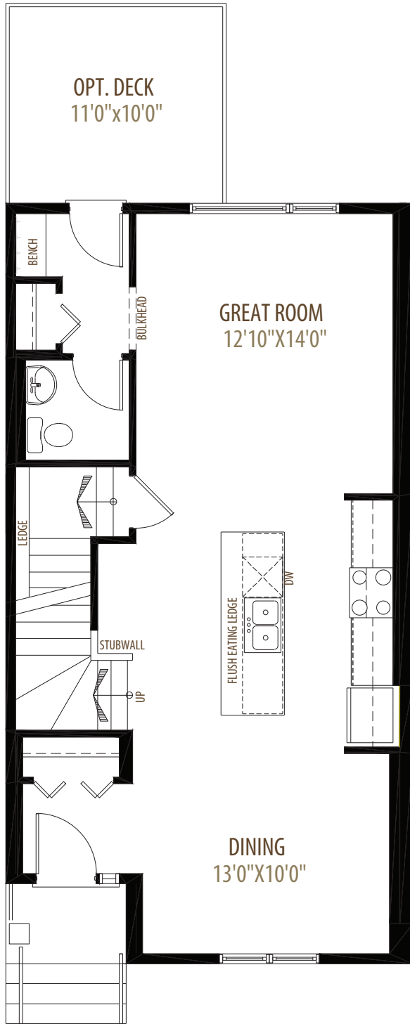
Main Floor 736 sq ft
