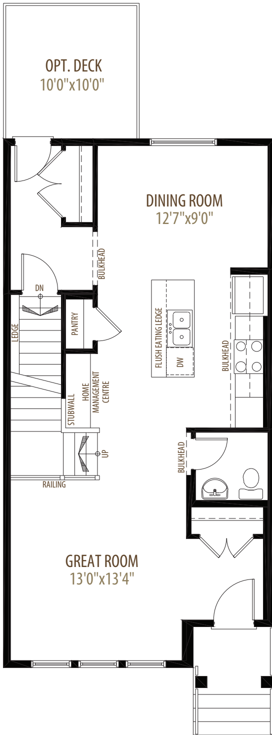
Main Floor 762 sq ft
